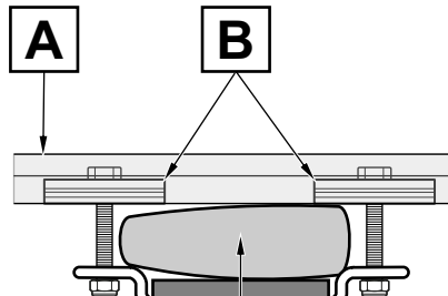
ROOFTOP TENT MOUNT BRACKET FOR VEHICLE CROSS BARS 2616041
